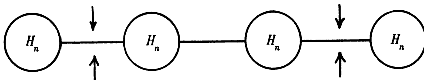
FIGURE 2. Selecting faces for m_{n+1} even
