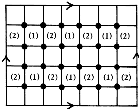
FIGURE 4. An imbedding of C_4 \times C_8 in the torus
